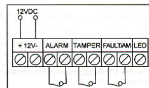
Figure 4. Schematic of EOL resistors
