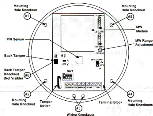
Figure 3. Terminal Wiring
